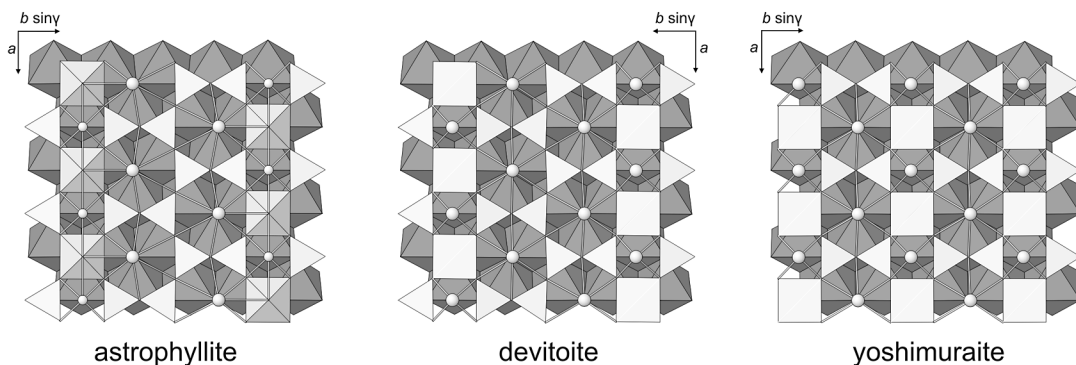
FIG. 6. Comparison of the sheet configurations in astrophyllite (LAB of Pilonen et al. 2003b), devitoite and yoshimuraite (McDonald et al. 2000), viewed perpendicular to the sheets.
