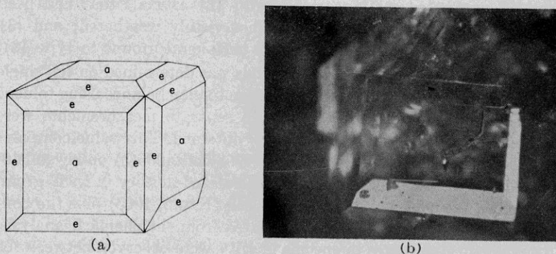
FIG. 2. Modification of melanophlogite cubes.
